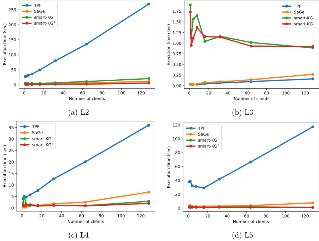
Figure 6.14: Avg. execution time per client on the standard WatDiv-100M, for simplest L queries
