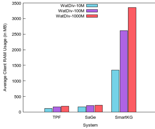
(b) Average Client RAM Usage (in MB)
