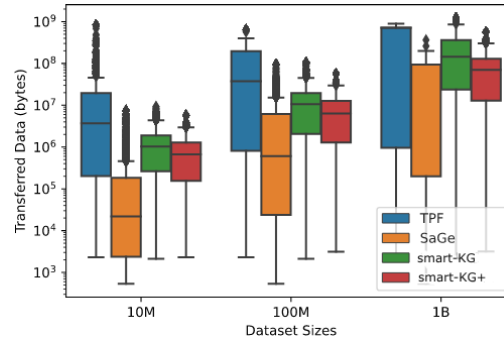
(a) Box plot summary for transferred data per query for the 128 clients over watdiv10M, watdiv100M, watdiv1B on watdiv-sts workload (log scale)
