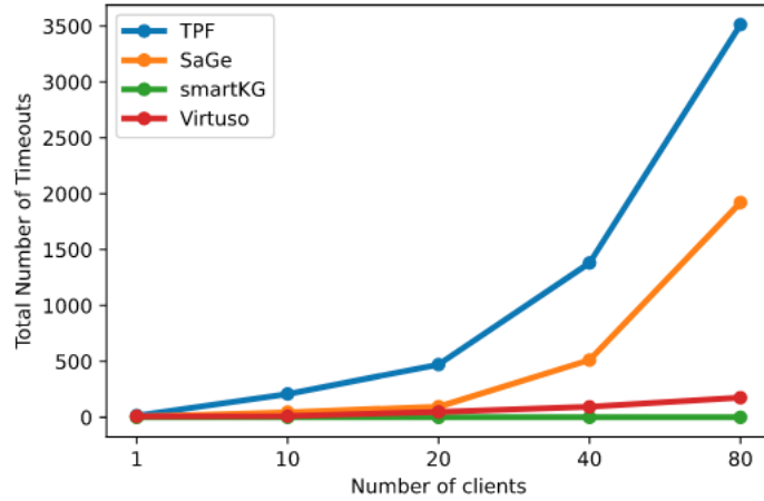
(a) Number of timeouts
