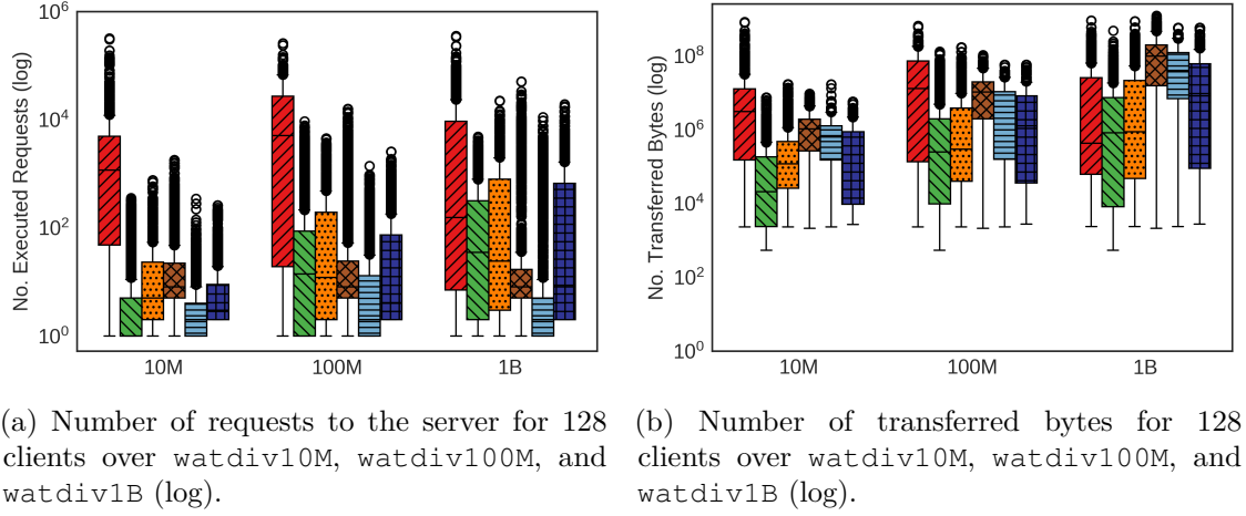
Figure 5.6: Number of requests to the server and number of transferred bytes for 128 clients over watdiv10M, watdiv100M, and watdiv1B, and CPU load for increasing numbers of clients over watdiv1B on the watdiv-sts workload
