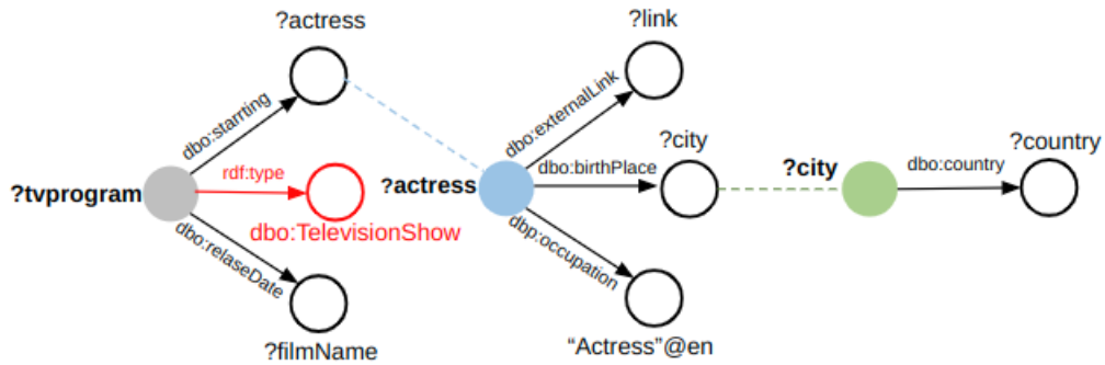
(b) Star-shaped query decomposition.
