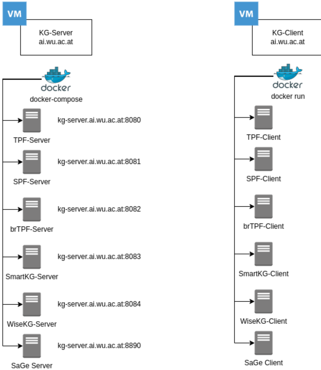
Figure 8.1: An illustration of our experiments infrastructure
