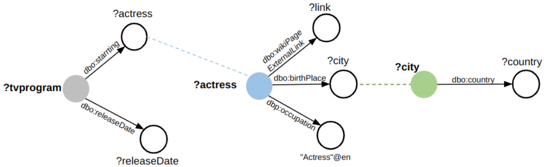
(b) Star-shaped query decomposition
