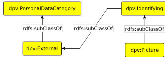
Fig. 2. Hierarchy of concepts for classifying depictions of individuals in pictures (inspired by EnterPrivacy [9])
